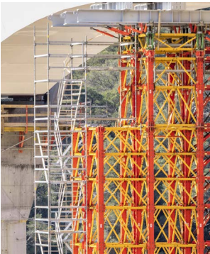
The PERI UP Stair Tower provided a safe and convenient means of access to the top.
