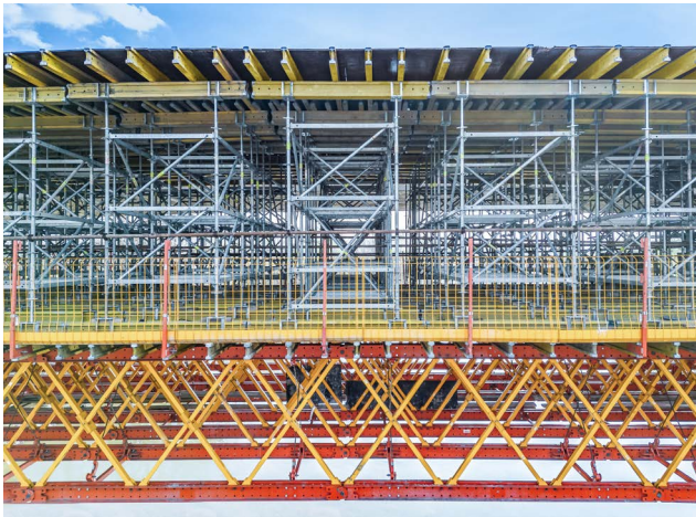
A well-thought-out combination of PERI System Solutions made it possible to construct the spans efficiently.
