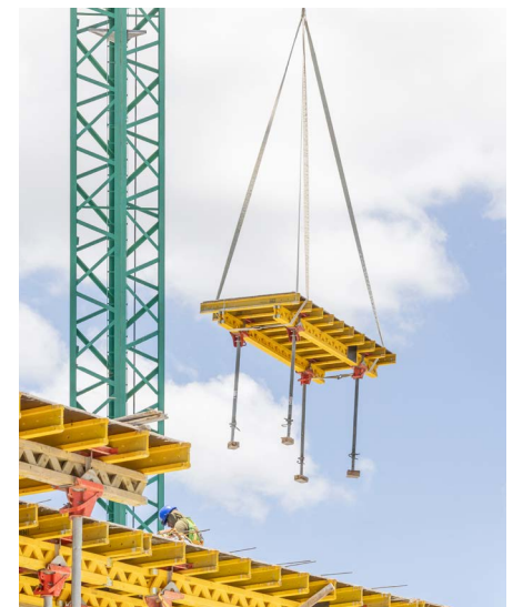
The choice of props and the customisation options offered by the VARIOKIT System Components ensured flexibility of design.
