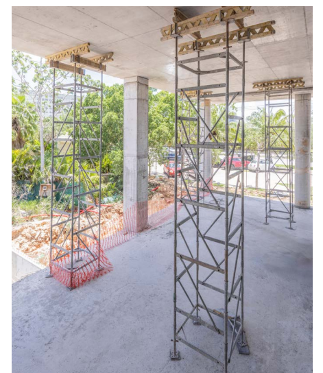
The ST 100 System was assembled using plug-in connections. As such, there was no need for connecting bolts or other parts that could easily go missing on the construction site.
