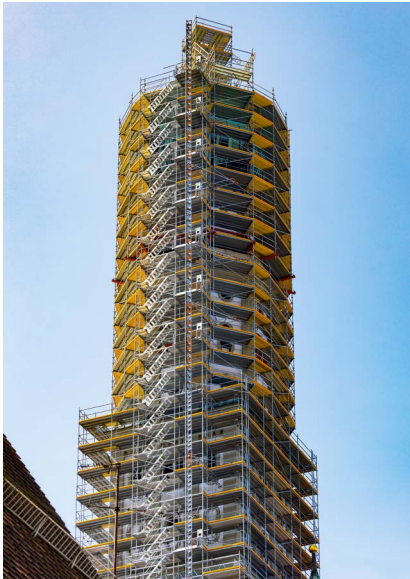
The transition from a square to octagonal cross-section halfway up the tower presented engineers with a unique challenge that was ultimately solved with the use of a PERI UP Scaffolding Kit.
